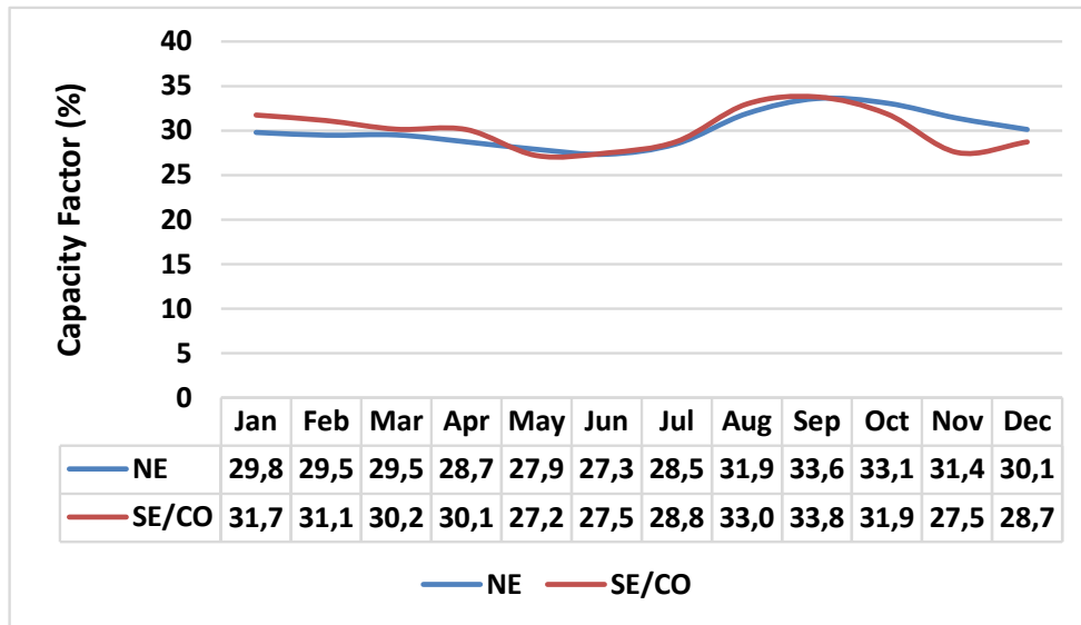
Figure 19 – Photovoltaic: Monthly capacity factor per subsystem
