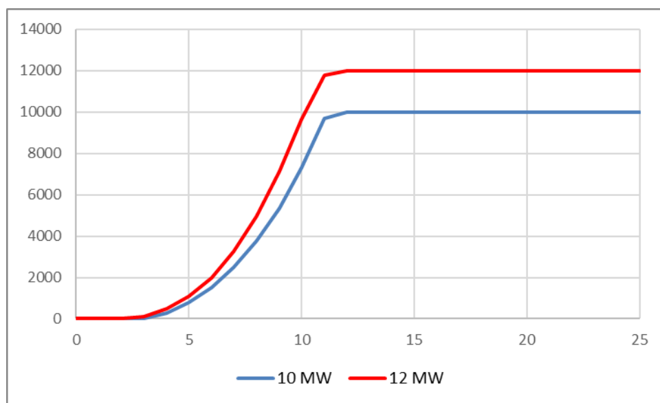
Figure 8 – Offshore turbines: power curves
