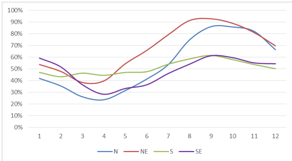
Figure 18 – Offshore wind: Monthly behavior
