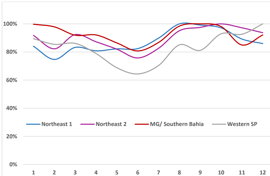
Figure 10 – Example of monthly profile by region
