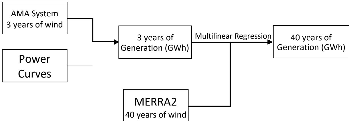
Figure 7 – Onshore wind – Flowchart
